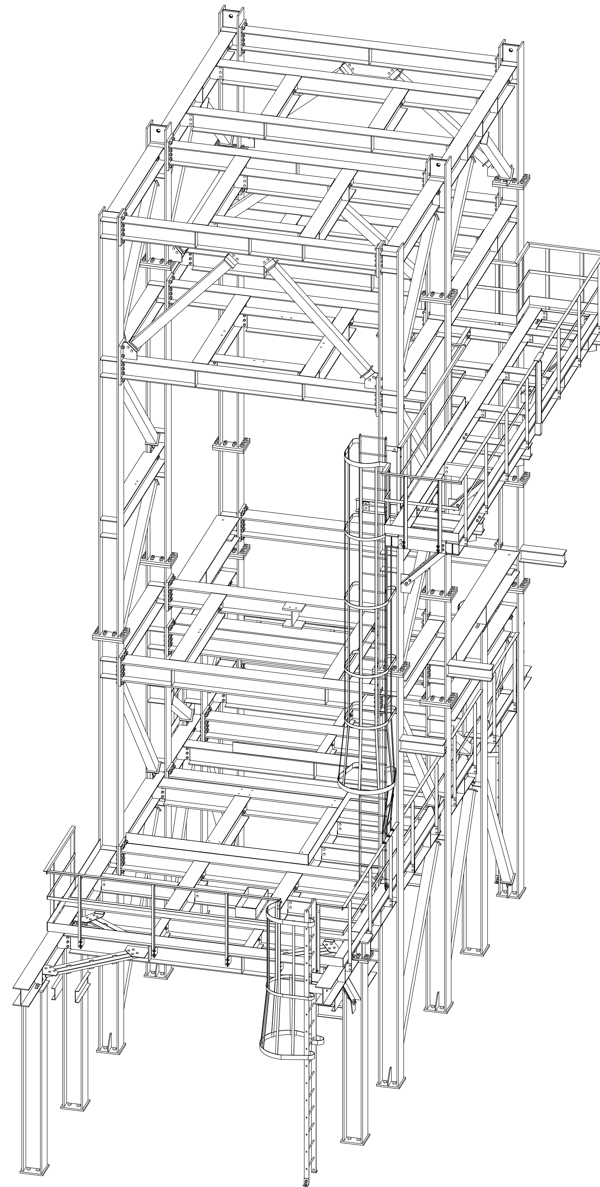
South-Isometric Views
