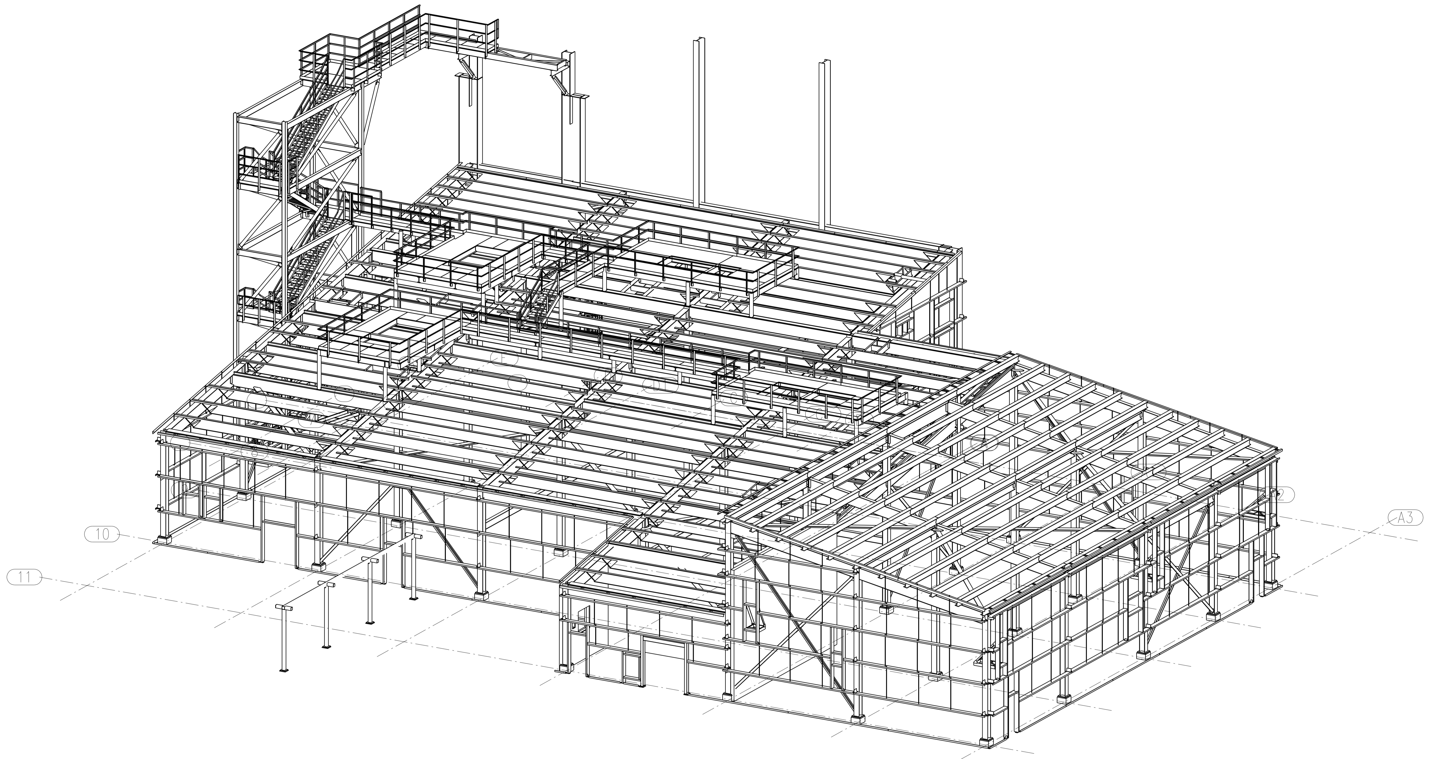
PERSPECTIVE VIEW (LOOKING SOUTH - WEST)
