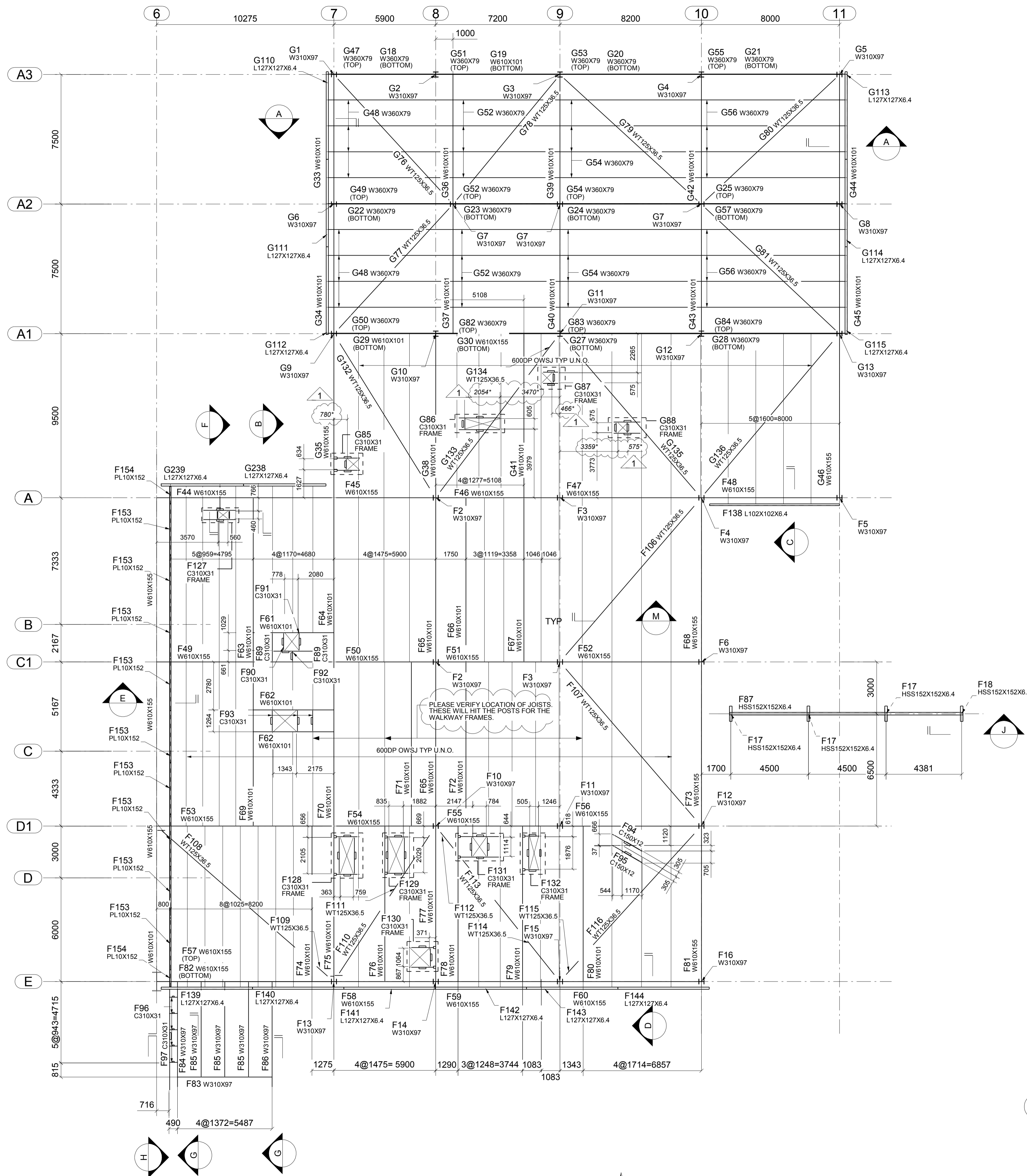
ROOF FRAMING PLAN
