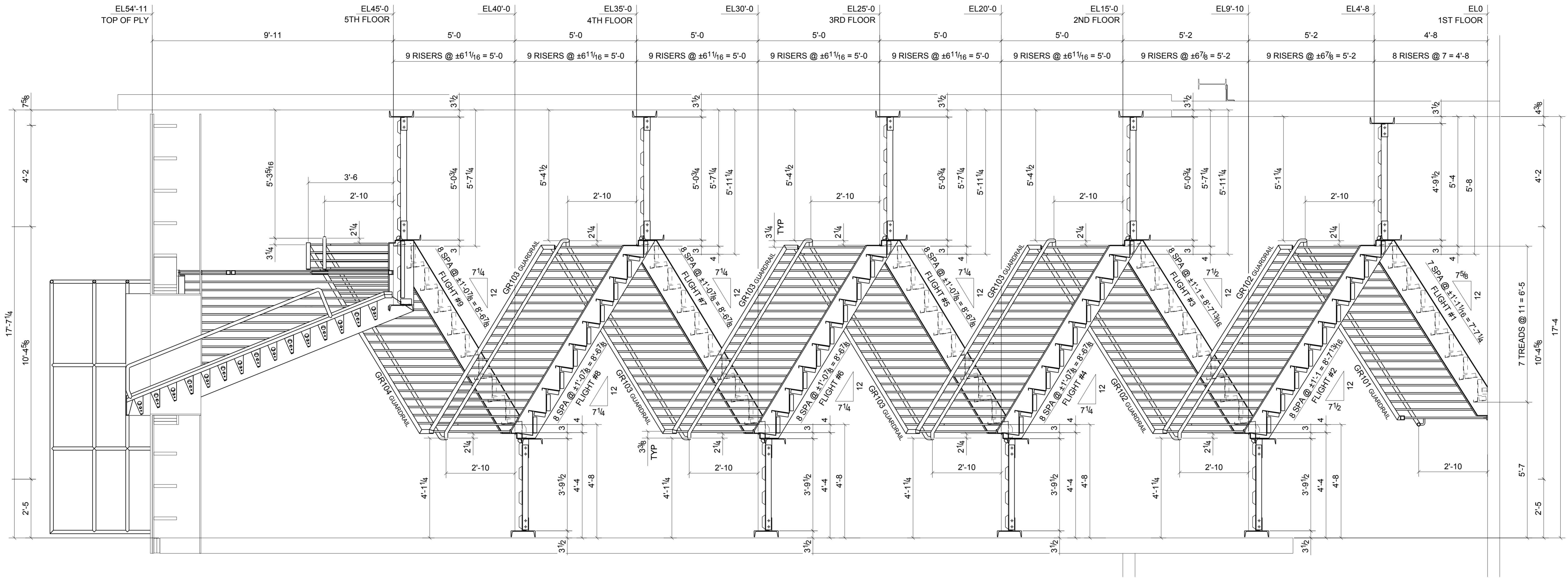
ELEVATION "1 - 1"
