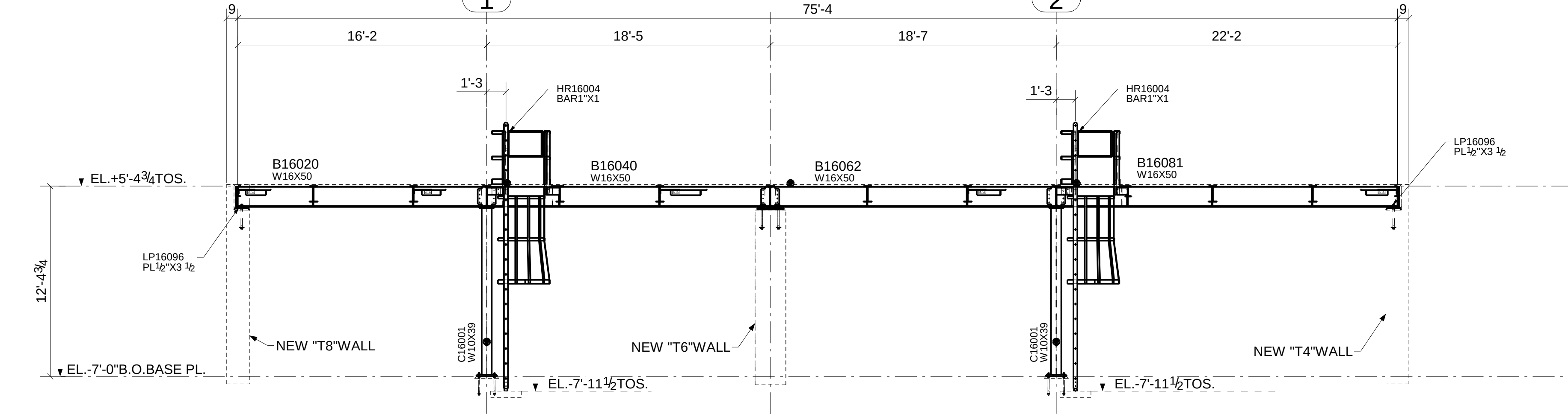
ELEVATION @ COL. LINE C
